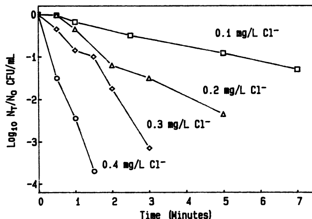
FIG. 3. Reduction of L. pneumophila by exposure to electrolytically generated copper and silver (400 and 40 \mu\text{g/liter} ) and various concentrations of free chlorine.
