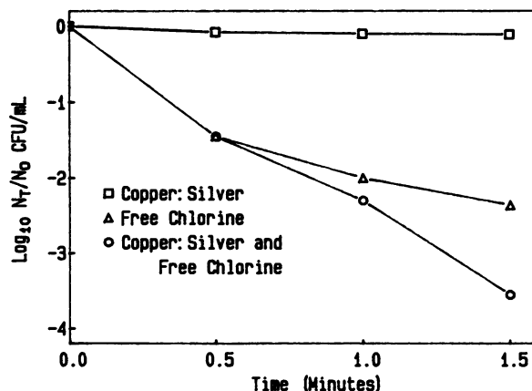
FIG. 4. Reduction of L. pneumophila by exposure to electrolytically generated copper and silver (400 and 40 \mu\text{g/liter} ) and/or free chlorine (0.4 \text{mg/liter} ).
