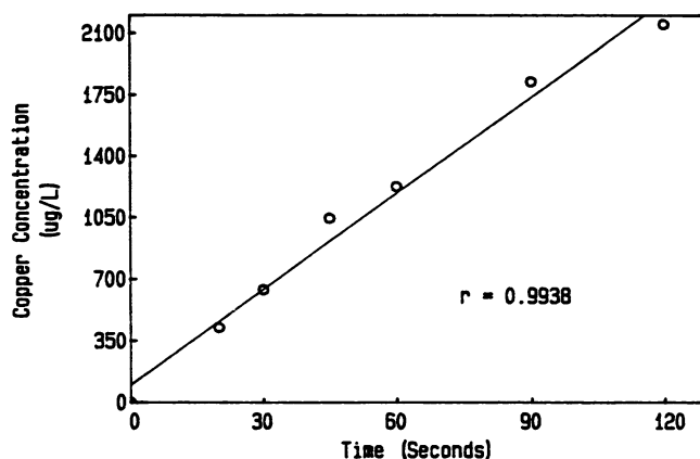
FIG. 1. Concentration of electrolytically generated copper in well water at room temperature with the 90:10 copper-silver unit.
