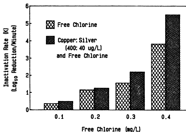
FIG. 2. Inactivation of L. pneumophila by exposure to electrolytically generated copper and silver (400 and 40 \mu\text{g/liter} ) and/or various concentrations of free chlorine.
