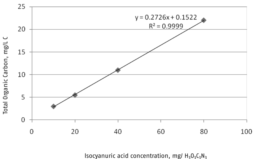
Figure 2 Correlation between TOC and isocyanuric acid concentration
