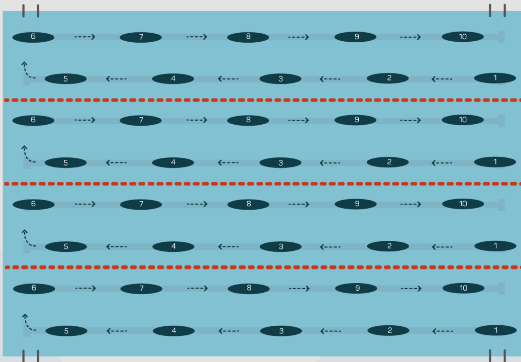
25x16.5m pool 10 to a double lane
