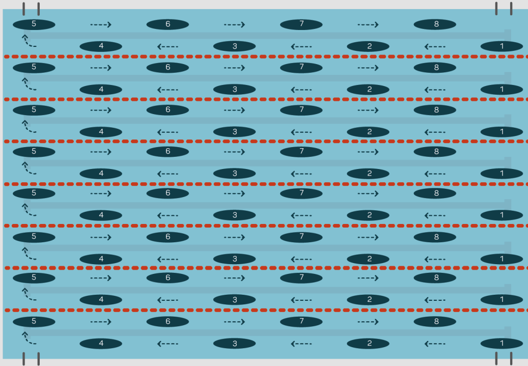
25x16.5m pool 8 to a single lane
